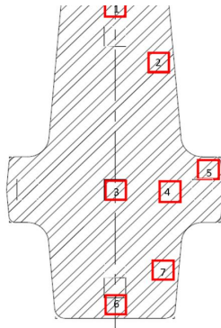
Fig. 8 Grain size sample location map.
