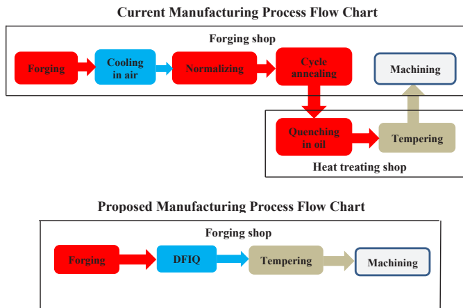
Fig. 5 Pintle adapter manufacturing process flow chart.
