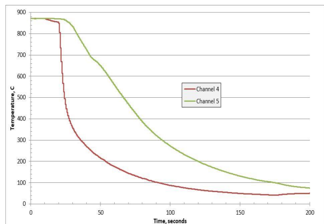
Fig. 11 Example of cooling curve.
