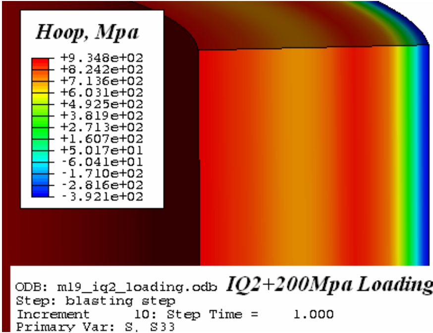
Figure 2.37 Hoop Stress with the Additional Pressure of 200 MPa Applied on the Bore Surface for the M19 Steel Barrel Intensively Quenched Only on the OD Surface.
