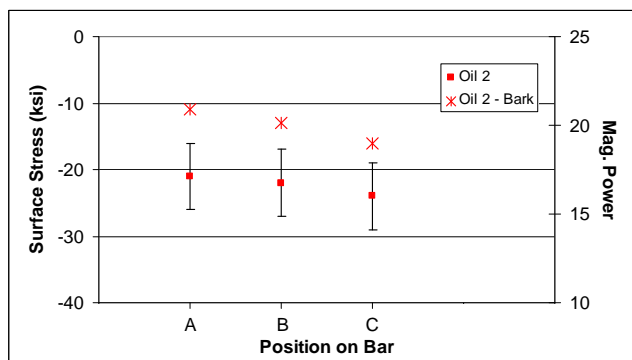
Figure 3.10 Comparison of Calculated X-Ray and Measured BN Response by Location on OQ Coupon #5
