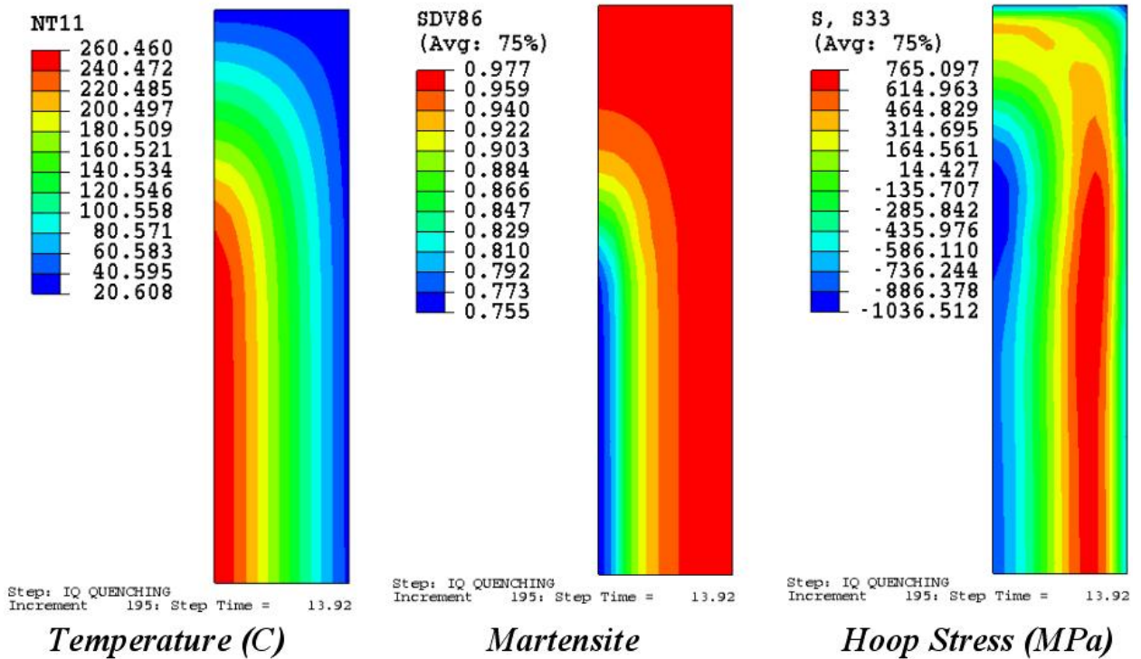
Figure 2.18 Profiles of Temperature, Martensite and Hoop Stress at the Time of Maximum Tensile Stress in Quenched Piece for Model 2
