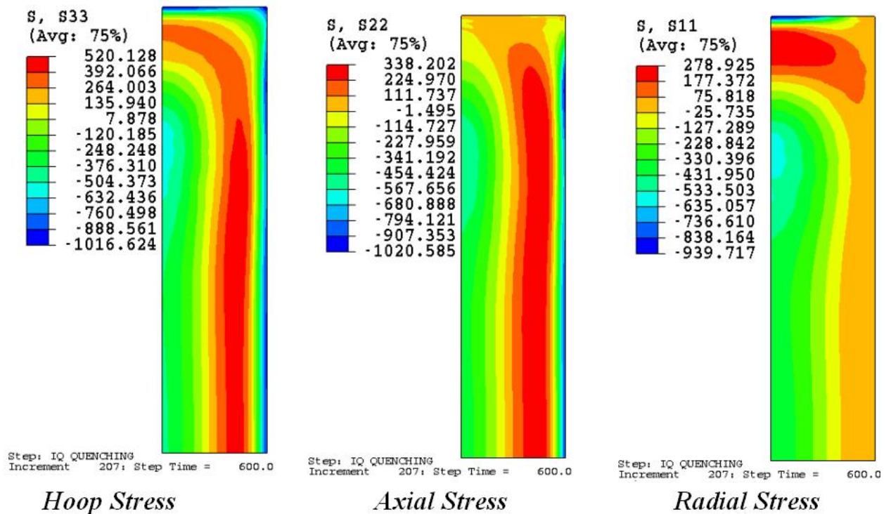
Figure 2.28 Predicted Residual Stress State for Model 6
