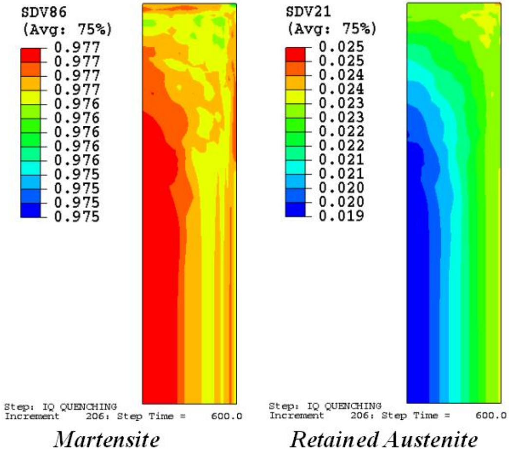
Figure 2.27 Predicted Metallurgical Phase Distributions After Intensive Quenching for Model 5
