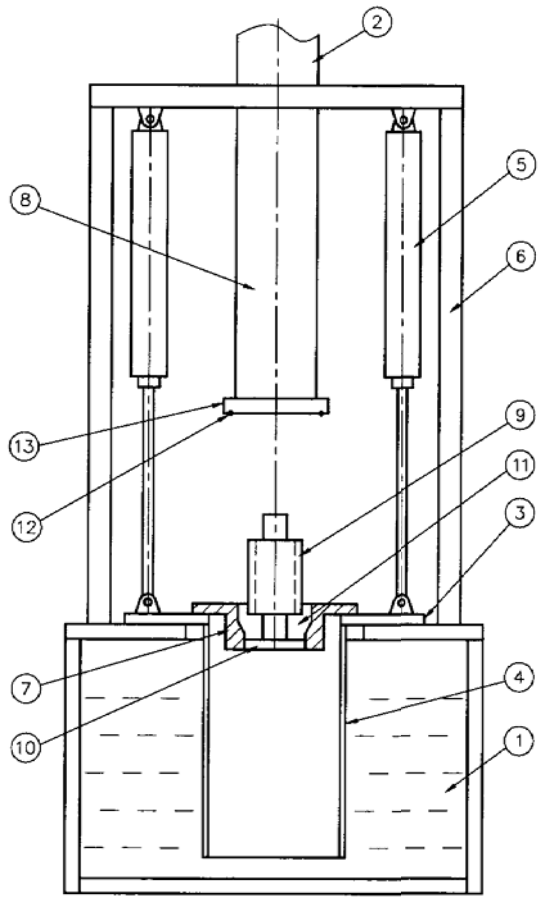
Figure 3.20 Layout of IQ Unit for Free Quenching of Gears
