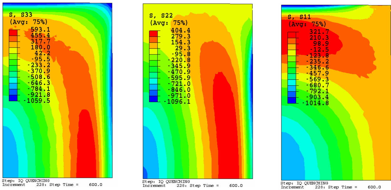
Hoop Stress
