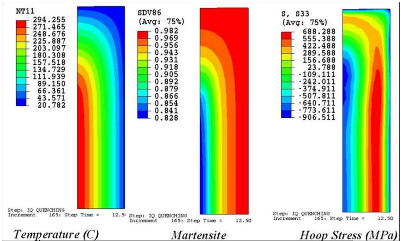
Figure 2.23 Profiles of Temperature, Martensite and Hoop Stress at the Time of Maximum Tensile Stress in Quenched Piece for Model 4
