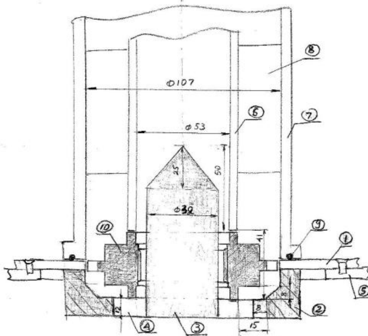
Figure 3.13 Schematic Showing the Test Gear In the Intensive Quench Station.
