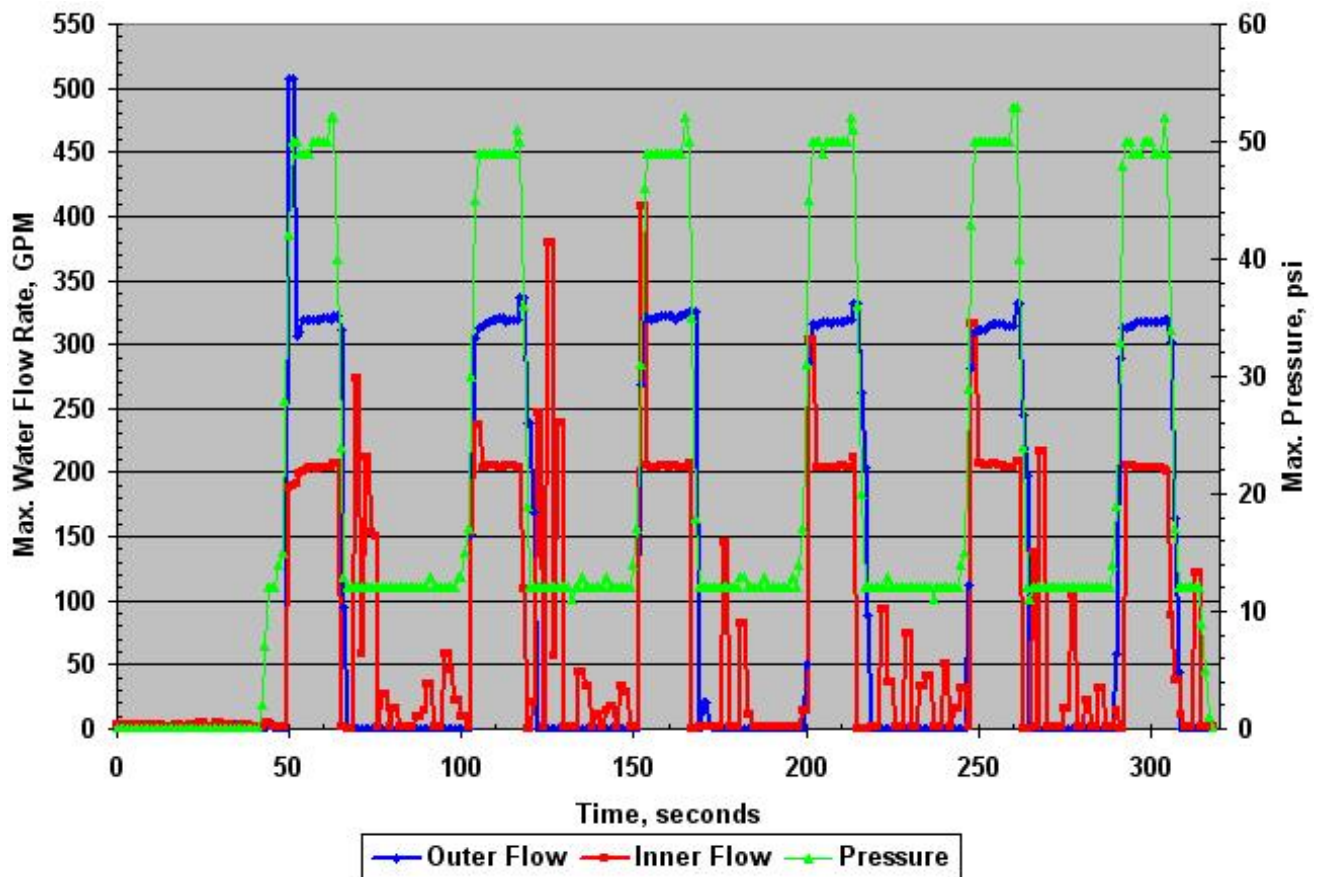
Figure 3.16 Plotted Data for Intensive Quenching 6 Test Gears. The Water Flow Rates in the Outer and Inner Tubes are 325 GPM and 205 GPM, respectively.
