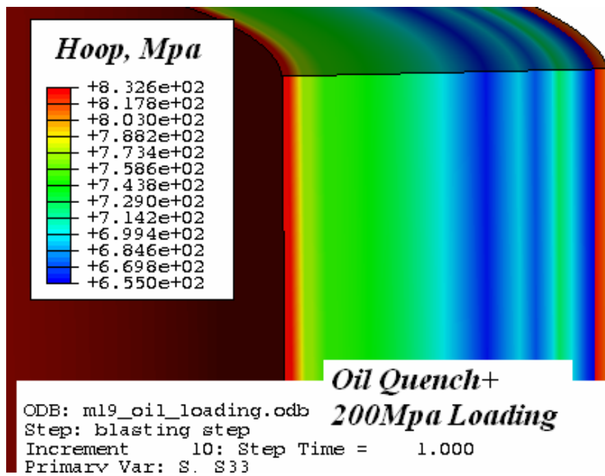
Figure 2.33 Hoop Stress Generated in Oil Quench Hardened Barrel for an Inner Barrel Pressure of 200 MPa.
