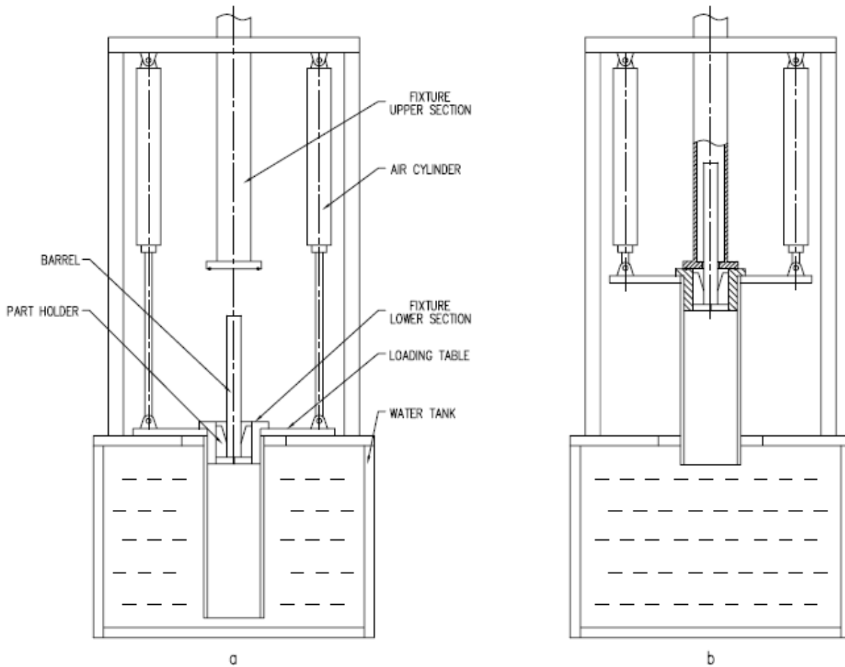
Figure 2.11 IQ Unit for Processing Small Gun Barrels
