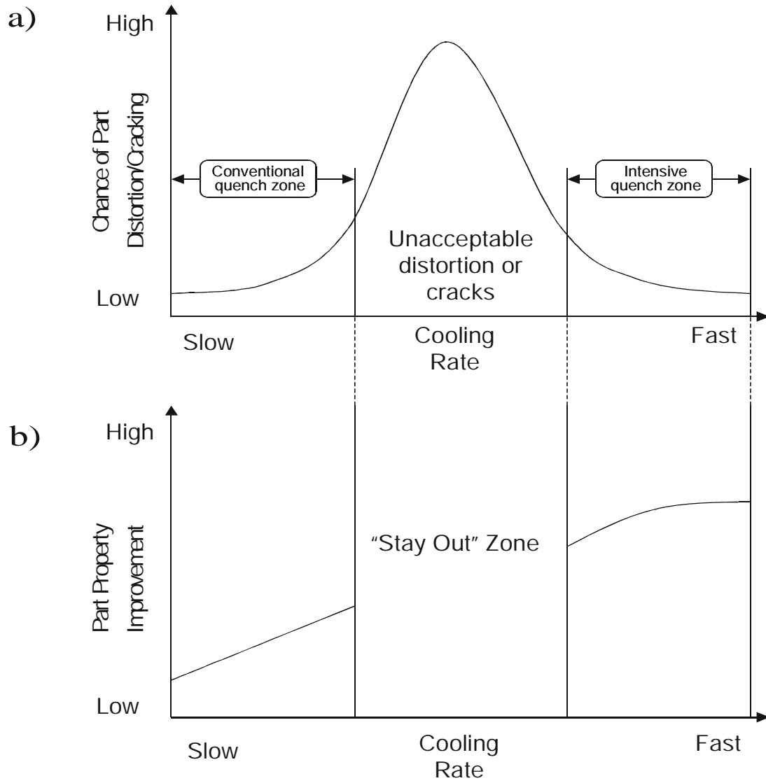
Figure 1 Intensive Quenching Phenomenon
