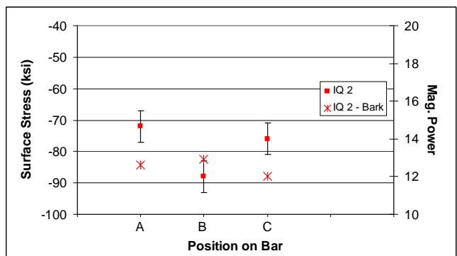
Figure 3.7 Comparison of Residual Stress Calculated from XRD and BN Measurements by Location on IQ Coupon #2
