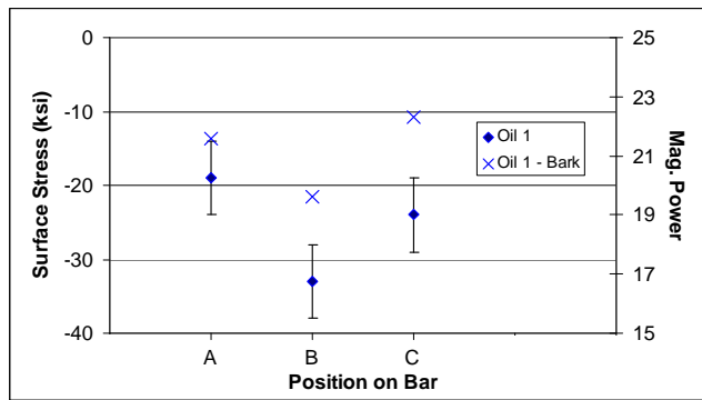
Figure 3.9 Comparison of Calculated X-Ray and Measured BN Response by Location on OQ Coupon #4
