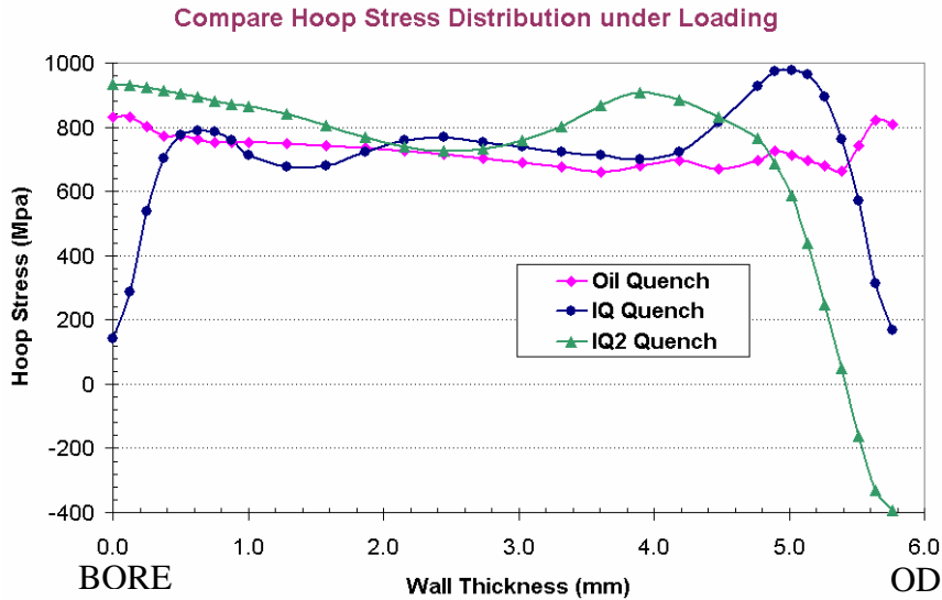
Figure 2.39 Hoop Stress Distribution for the Bore Pressurized Condition for the Oil Quenched or Intensively Quenched M19 Barrels.
