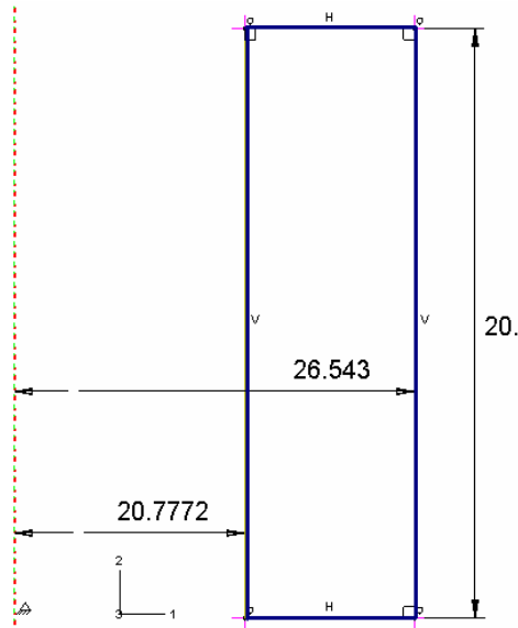
Figure 2.31 Cross Section of Small Caliber Barrel Used for the Baseline Quench Hardening and Ballistics Models.
