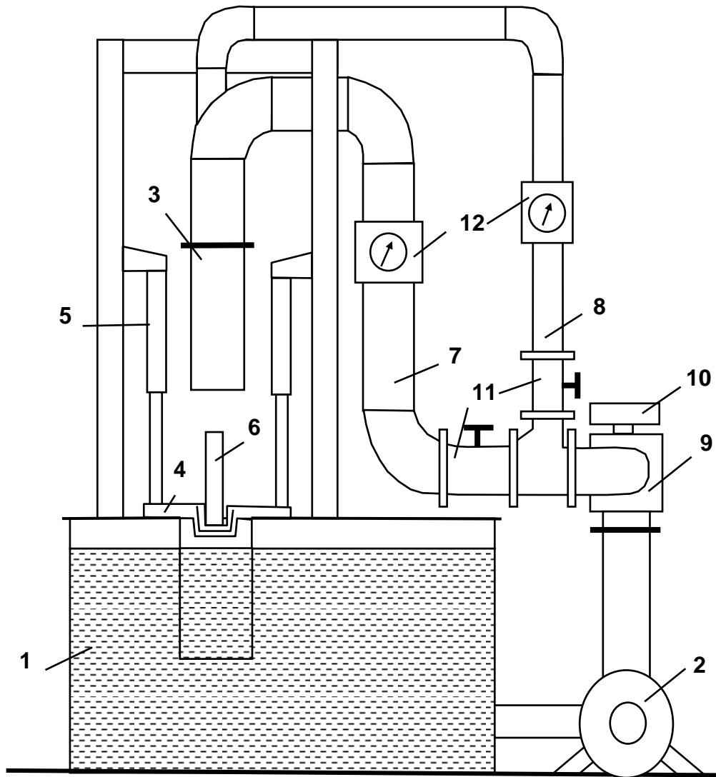
1 – 800-gallon quench tank; 2- 600-gpm pump; 3 – adjustable upper section of the fixture; 4 - loading table; 5 - four air cylinders and four linear bearings; 6 – part to be quenched; 7 and 8 - piping; 9 - 3-way solenoid valve; 10 – bypass pipe; 11 - shut-off valves; 12 – flow meters.
