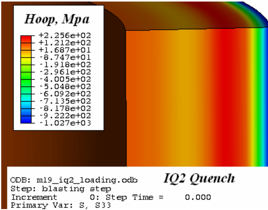
Figure 2.36 Predicted Hoop Stress for and M19 Steel Barrel Intensively Quenched Only on the OD Surface.
