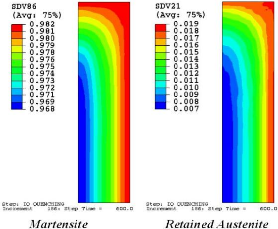
Figure 2.24 Predicted Metallurgical Phase Distributions After Intensive Quenching for Model 4
