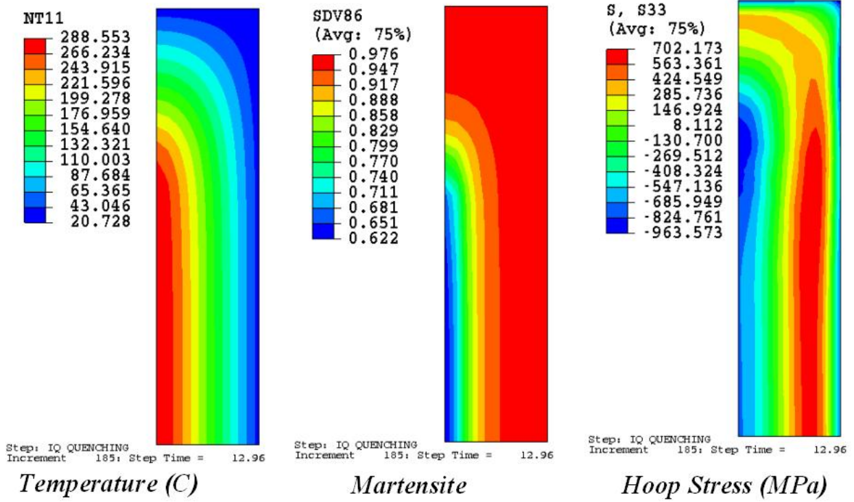
Figure 2.26 Profiles of Temperature, Martensite and Hoop Stress at the Time of Maximum Tensile Stress in Quenched Piece for Model 5
