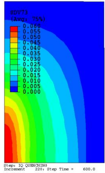
Lower Bainite
