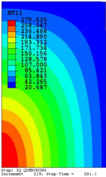
Temperature (C)
