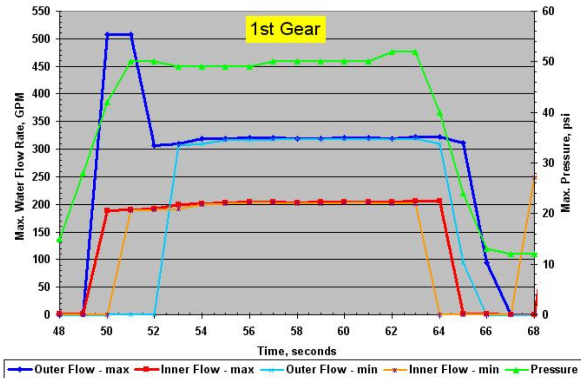
Figure 3.17 Intensive Quenching Process Data for the 1 st Quenched Gear from the Set Shown in Figure 3.6. Both Maximum and Minimum Flow Rates are Gathered, as well as the Pump Pressure.
