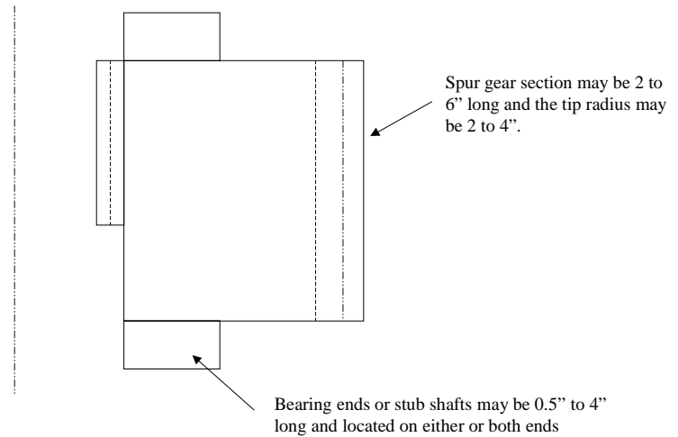
Figure 3.19 Helicopter Gears Suitable for Free Quenching
