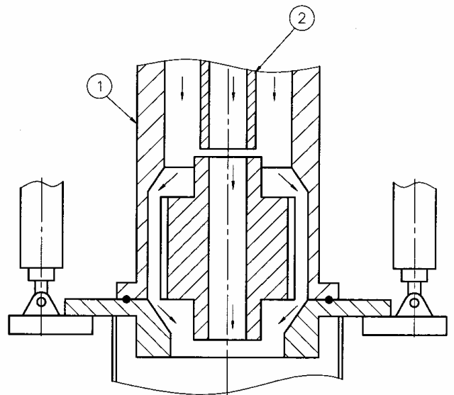
Figure 3.22 Quench Chamber Design Providing Axial Water Flow
