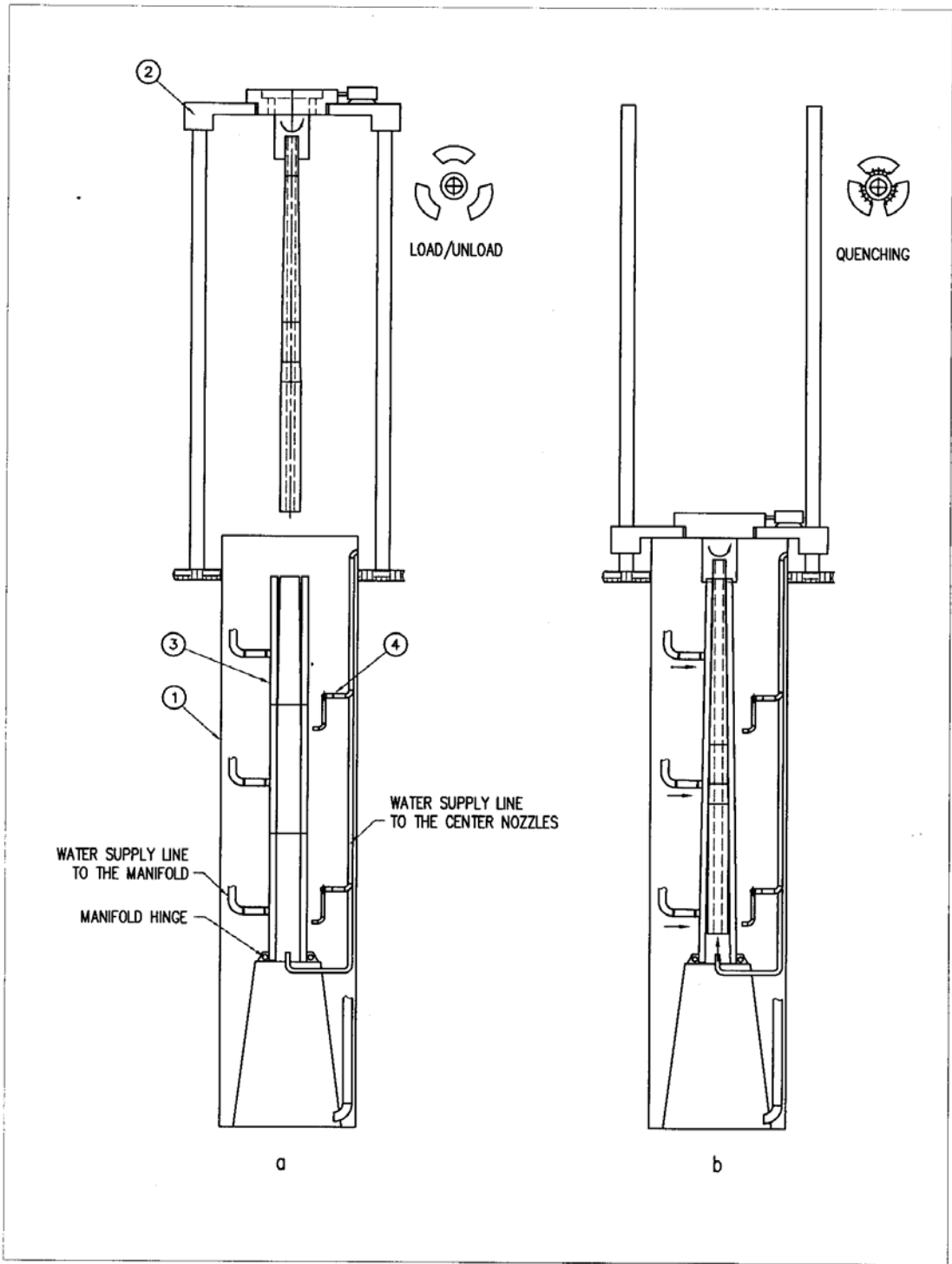
Figure 2.8 Quenching of Long Cannon Barrel in IQ System
