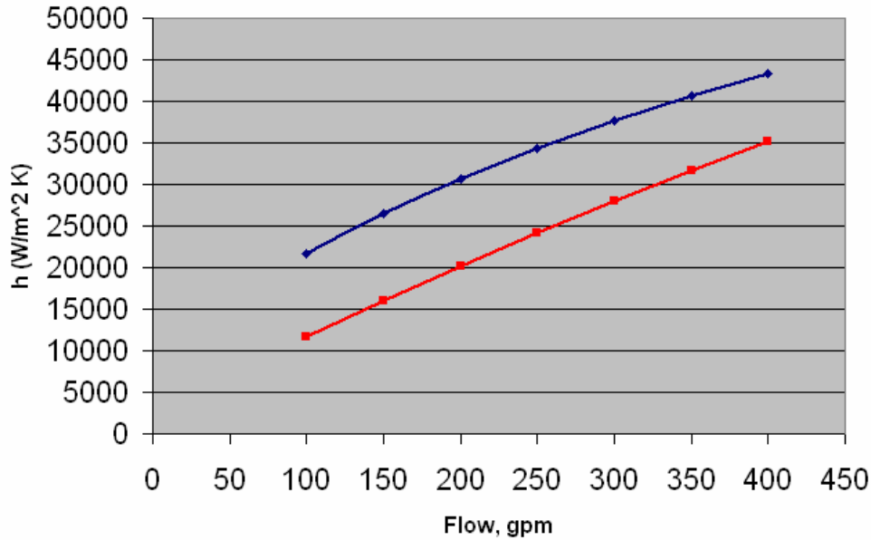
Figure 3.18. Heat Transfer Coefficients Calculated from Water Flow Rates Using Dimensionless Parameters.
