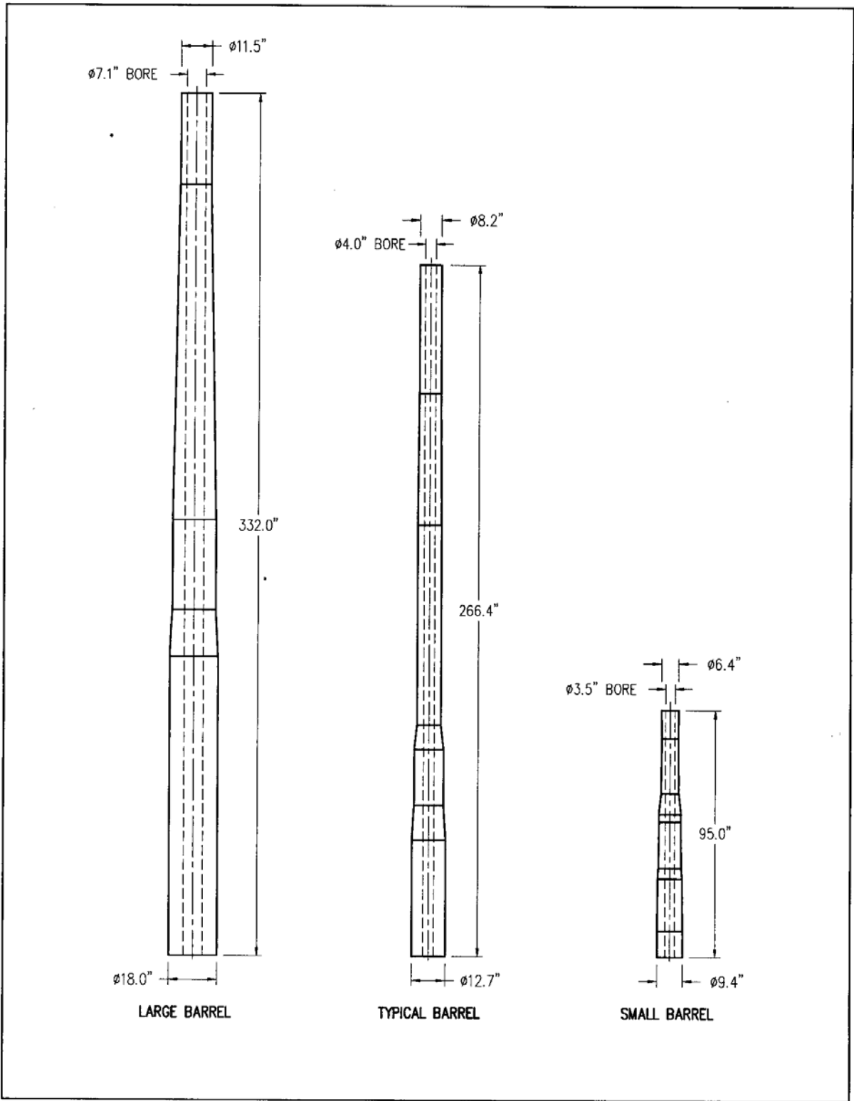
Figure 2.7 Large Caliber Cannon Barrel Sketches
