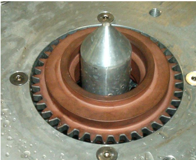
Figure 3.15 Cold Test Gear Loaded in the Intensive Quenching Station Showing the Water Flow Channels in the Bore and Around the Spur Teeth.
