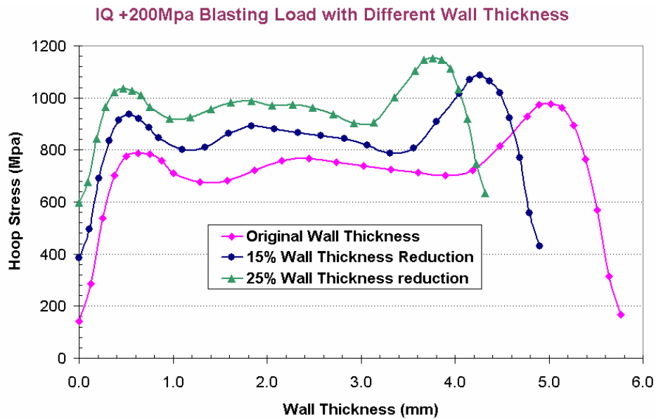
Figure 2.41 Predicted Hoop Stress Resulting from a 200 MPa Bore Pressure Applied to Intensively Quenched Barrels of Baseline Thickness (~5.8 mm Thick), 15% Thinner (~4.93 mm Thick) and 25% Thinner (~4.35 mm Thick) Wall Thickness.
