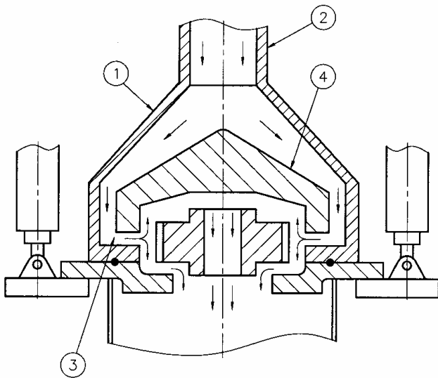
Figure 3.21 Quench Chamber Design Providing Radial Water Flow
