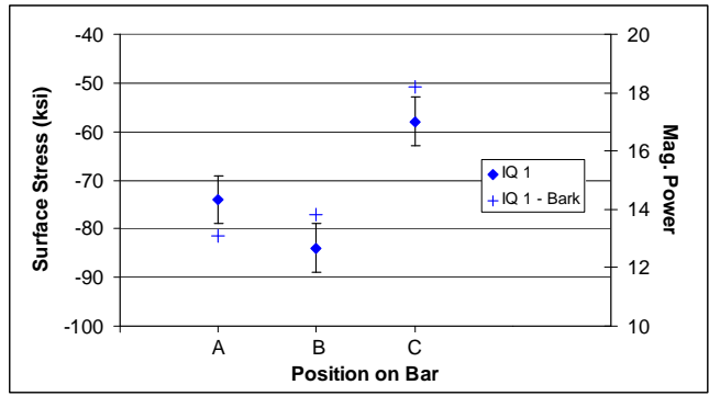
Figure 3.6 Comparison of Residual Stress Calculated from XRD and BN Measurements by Location on IQ Coupon #1
