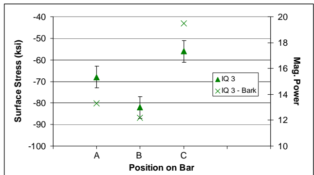
Figure 3.8 Comparison of Calculated X-Ray and Measured BN Response by Location on IQ Coupon #3
