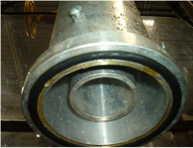
Figure 3.14 Photograph of the upper coaxial tubes showing the inner and outer tubes and the sealing gasket.
