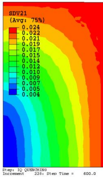
Retained Austenite
