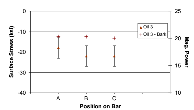
Figure 3.11 Comparison of Residual Stress Calculated from XRD and BN Measurements by Location on OQ Coupon #6
