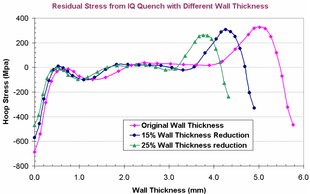
Figure 2.40 Predicted Residual Hoop Stress Resulting from Intensive Quenching of the Baseline Barrel (~5.8 mm Thick), 15% Thinner (~4.93 mm Thick) and 25% Thinner Barrels (~4.35 mm Thick).
