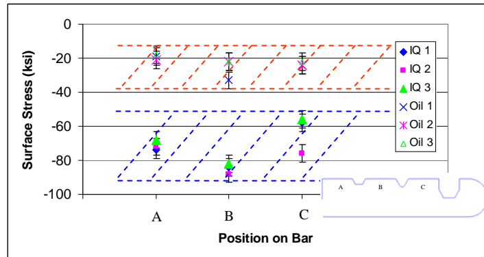
Figure 3.5 Comparison of Surface Residual Stress Variation at Three Locations on the Notched Specimens
