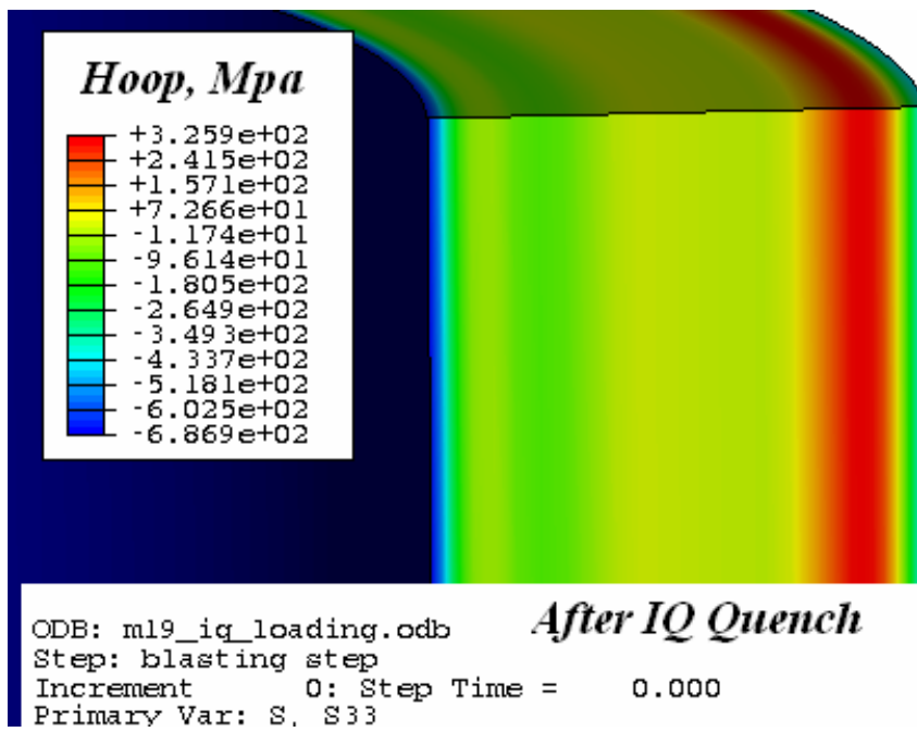
Figure 2.34 Predicted Hoop Stress for Intensively Quenched M19 Steel Barrel. Both ID and OD Surfaces are Quenched.
