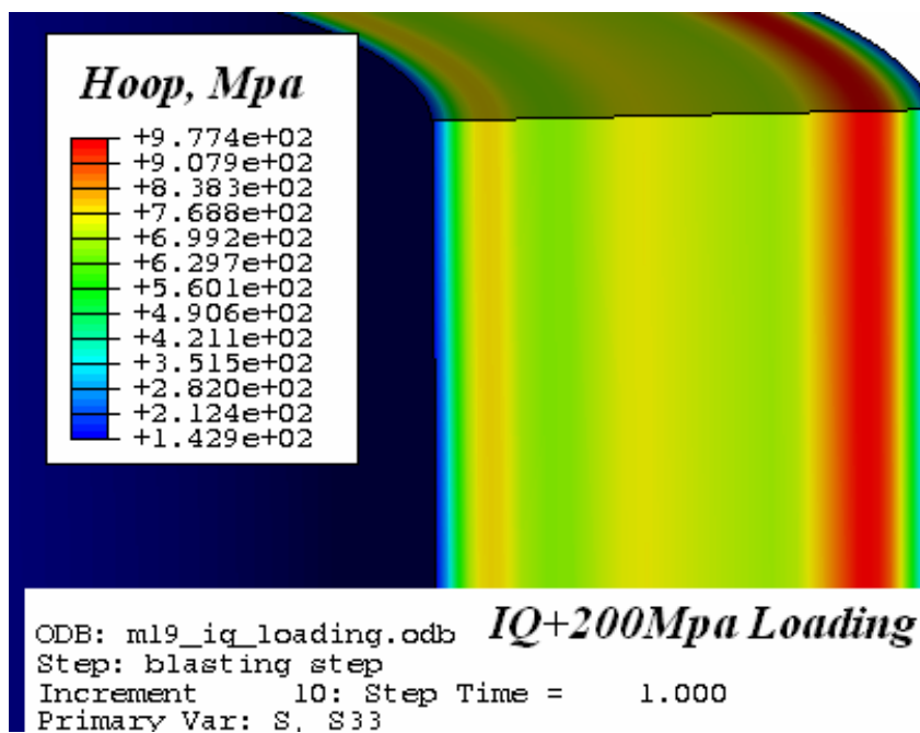
Figure 2.35 Hoop Stress with the Additional Pressure of 200 MPa Applied on the Bore Surface for the Intensively Quenched M19 Steel Barrel.
