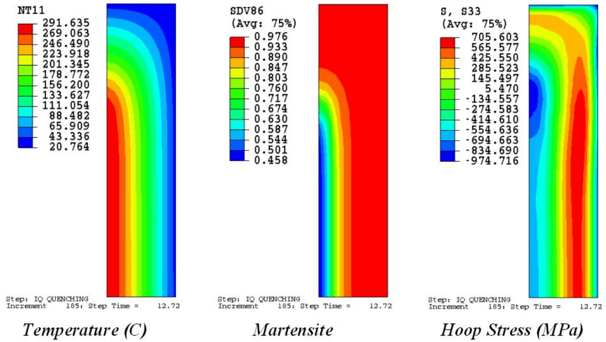
Figure 2.29 Profiles of Temperature, Martensite and Hoop Stress at the Time of Maximum Tensile Stress in Quenched Piece for Model 6
