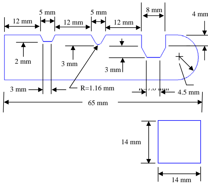
Figure 3.3 Schematic of Triple-Notched Bar Test Coupon Sensitivity Analyses
