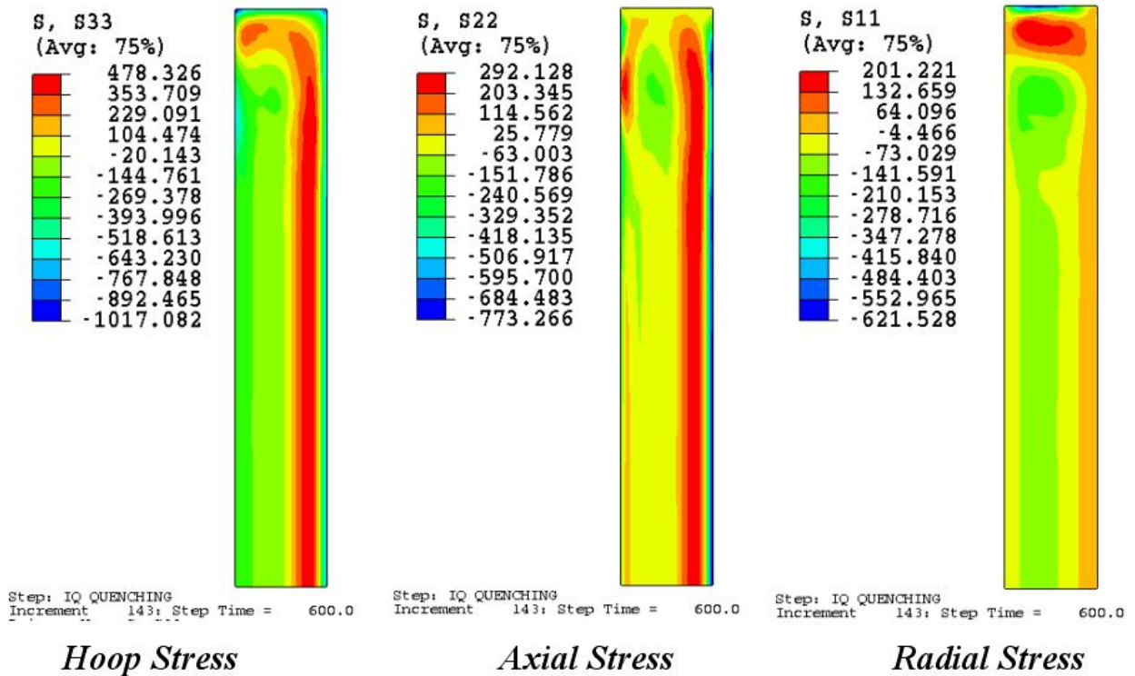
Figure 2.19 Predicted Residual Stress State for Model 3
