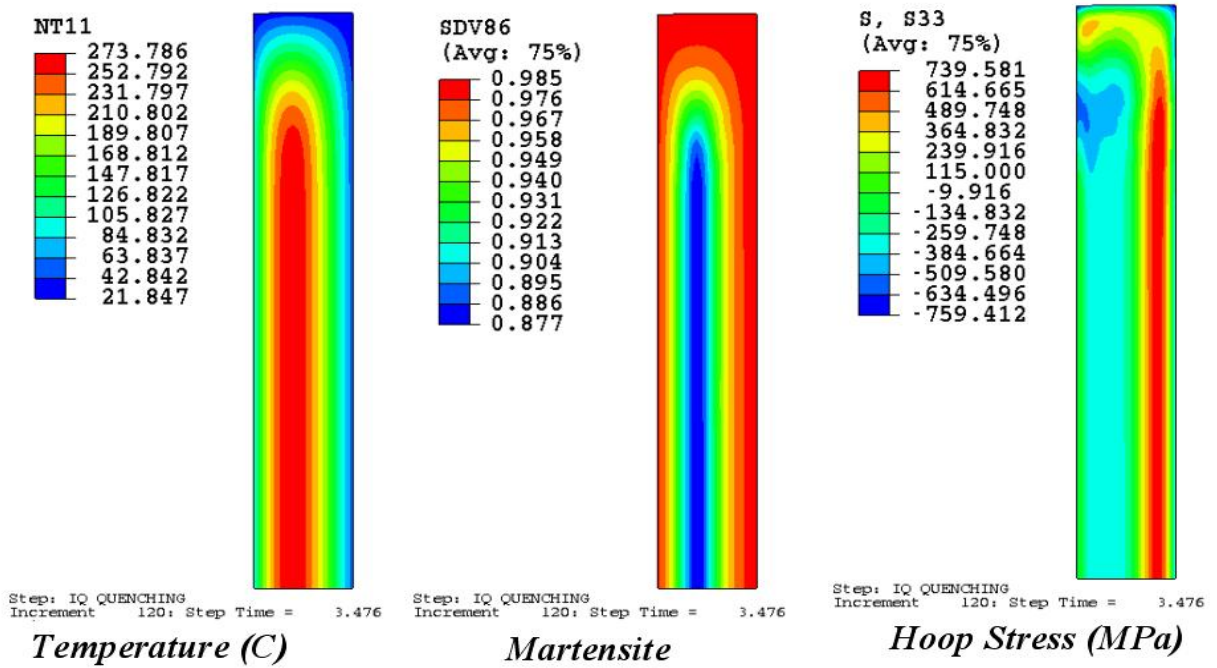
Figure 2.20 Profiles of Temperature, Martensite and Hoop Stress at the Time of Maximum Tensile Stress in Quenched Piece for Model 3
