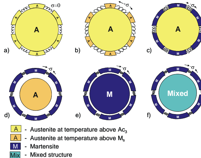
Figure 3 Surface Stress Conditions During Intensive Quenching.
