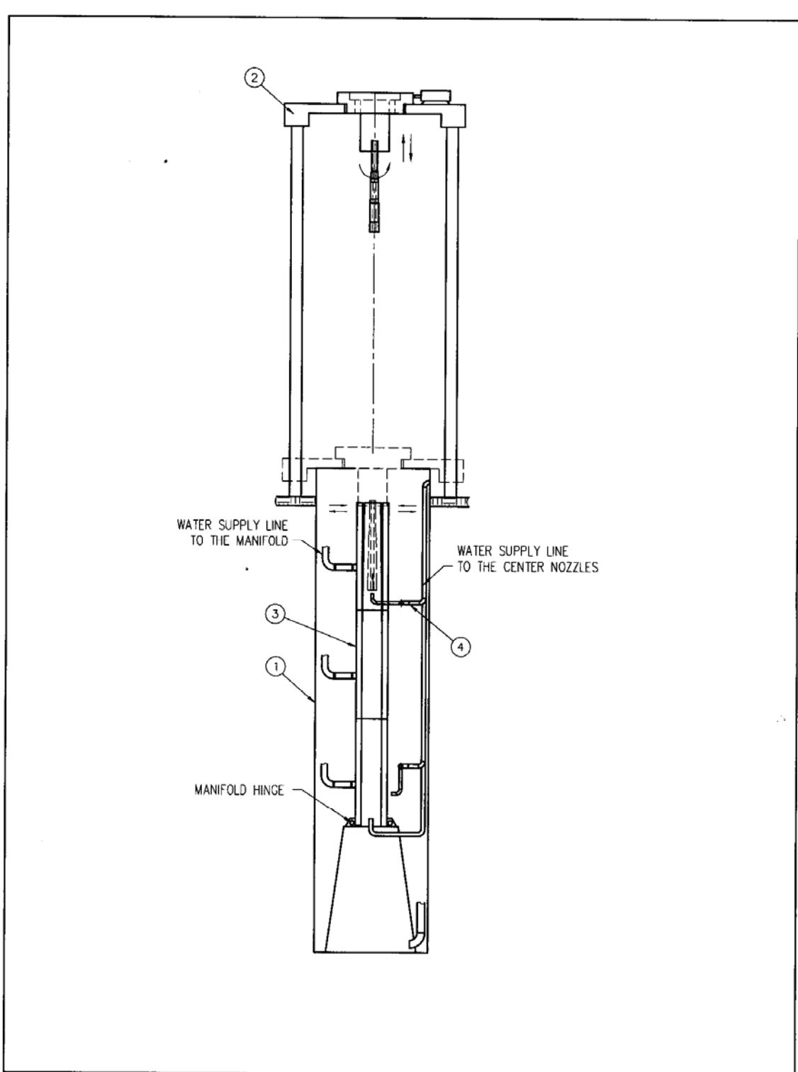
Figure 2.9 Quenching of Short Cannon Barrel in IQ System
