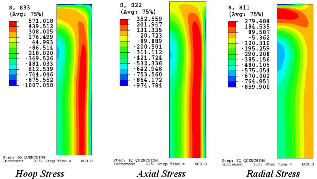
Figure 2.16 Predicted Residual Stress State for Model 2
