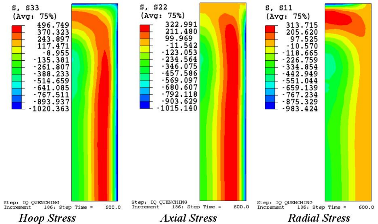
Figure 2.22 Predicted Residual Stress State for Model 4
