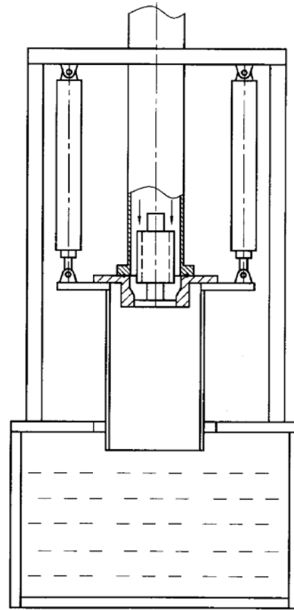
Figure 3.20 Layout of IQ Unit for Free Quenching of Gears
