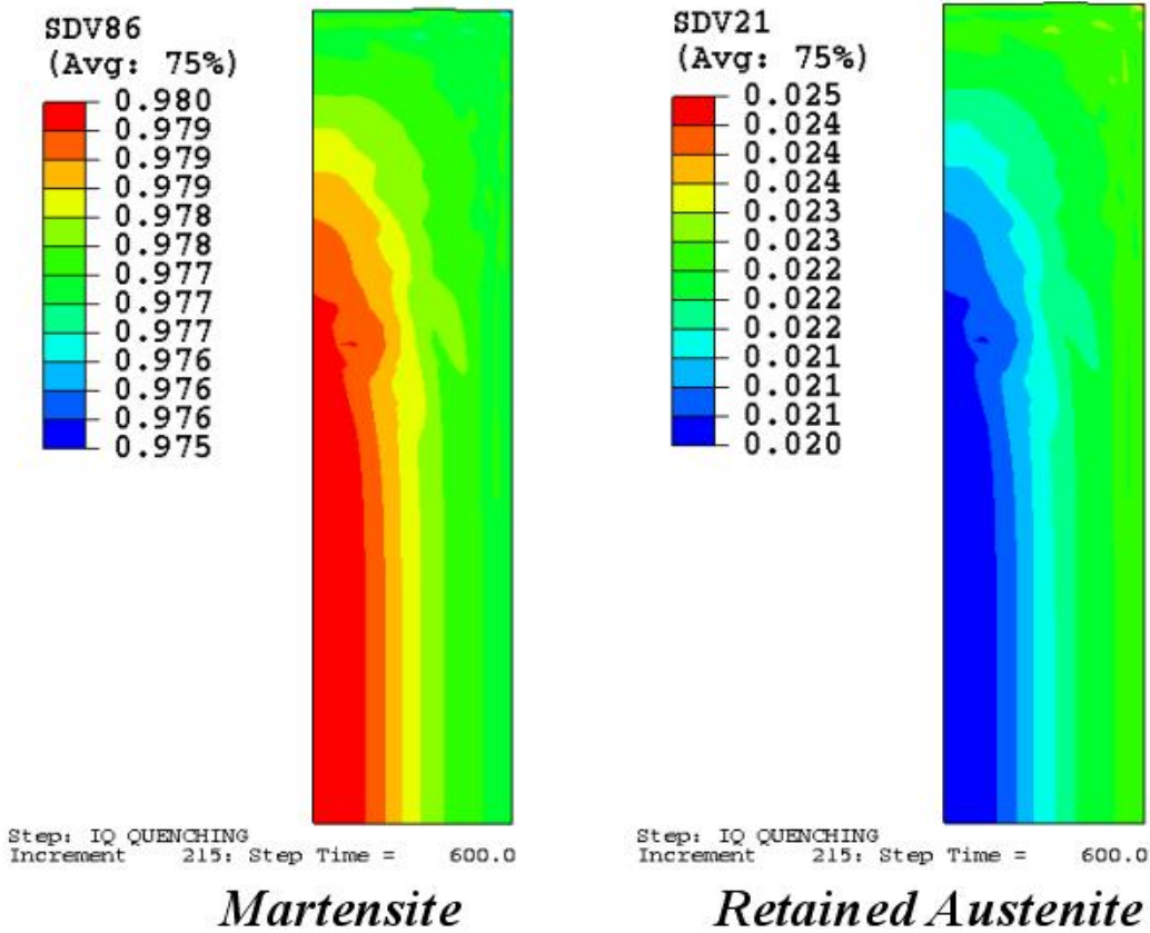
Figure 2.17 Predicted Metallurgical Phase Fractions for Model 2
