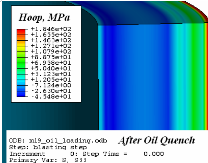
Figure 2.32 Hoop Stress Predicted for the Baseline Oil Quench Hardened M19 Barrel.
