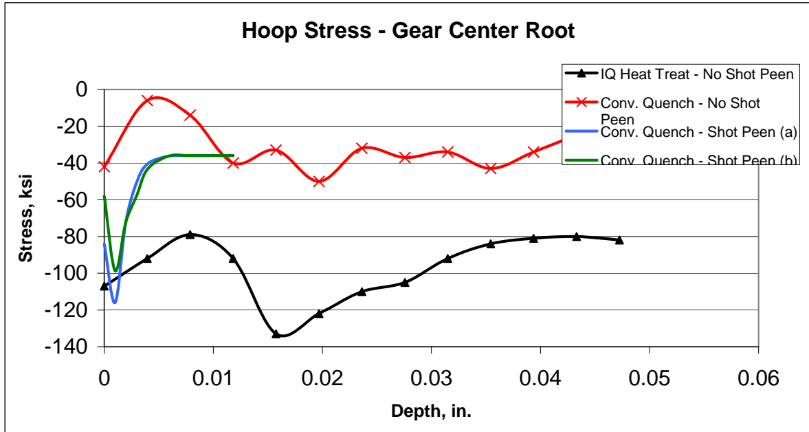
Figure 4 Hoop Stress Distribution in Test Gear
