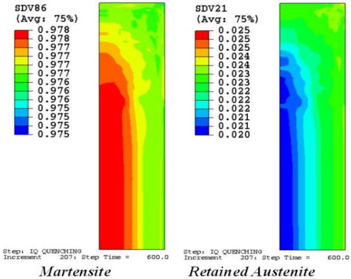
Figure 2.30 Predicted Metallurgical Phase Distributions After Intensive Quenching for Model 6
