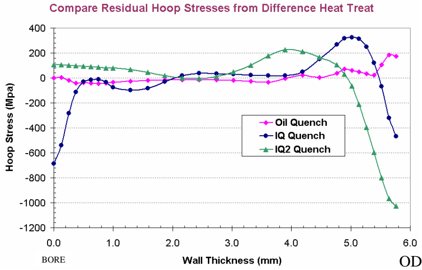
Figure 2.38 Predicted Hoop Stress Distribution from Bore to OD for the Oil Quenched and Intensively Quenched Conditions for the M19 Barrels.
