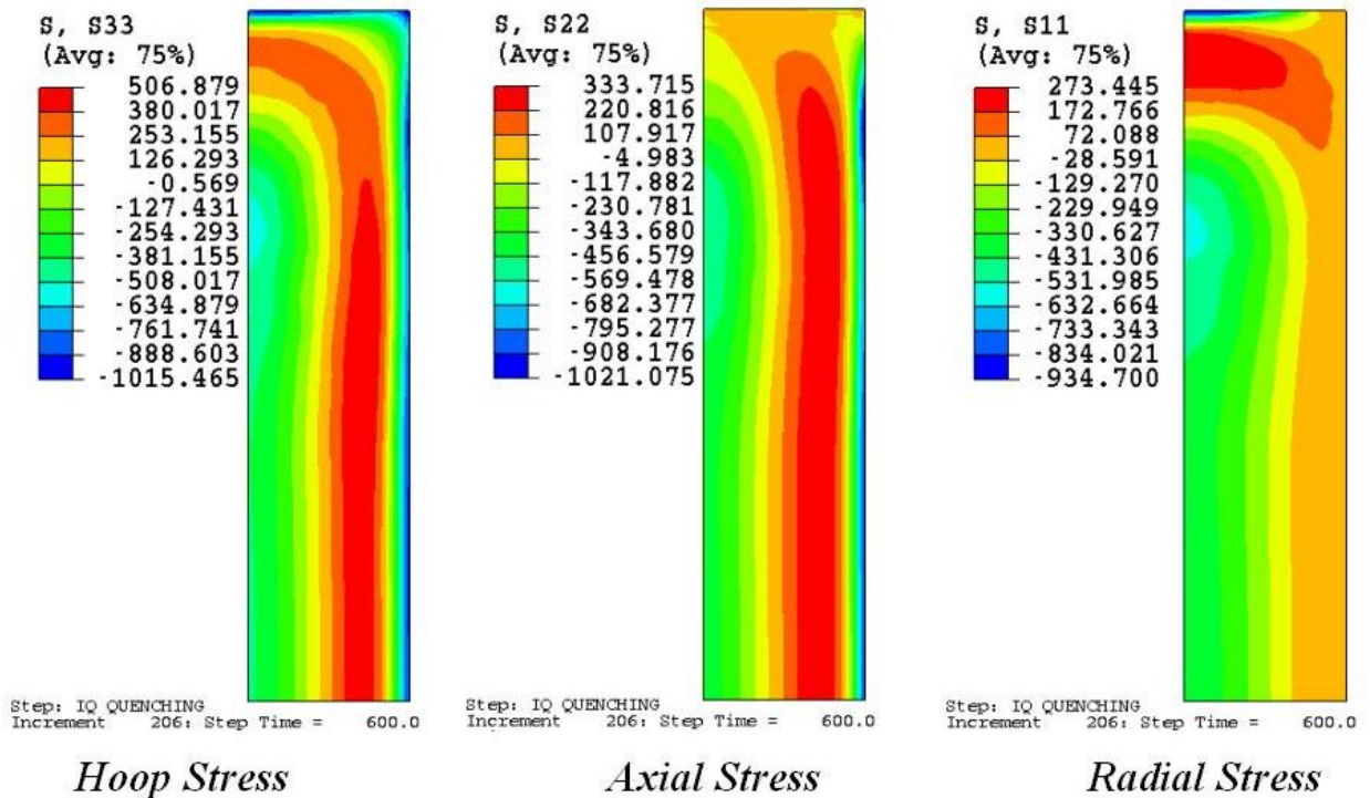
Figure 2.25 Predicted Residual Stress State for Model 5
