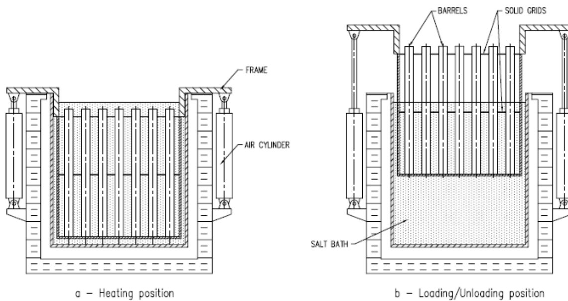
Figure 2.12 Furnace for Heating Small Gun Barrels with Loading/Unloading System
