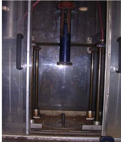
Figure 2.1 Fixture for Quenching Ø1"x5" Samples
